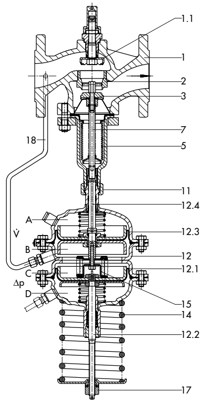
Fig. 3: Type 42-37 Flow and Differential Pressure Regulator (balanced by a bellows)
