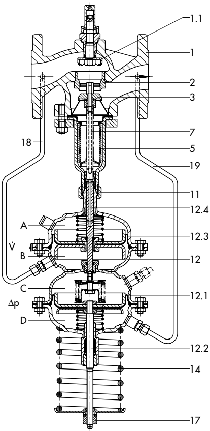
Fig. 4: Type 42-39 Flow and Differential Pressure or Pressure Regulator (balanced by a bellows)
