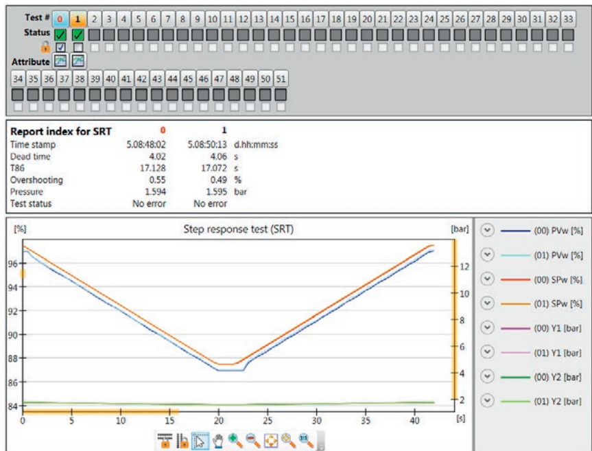
Fig. 9: Step response test (SRT)
